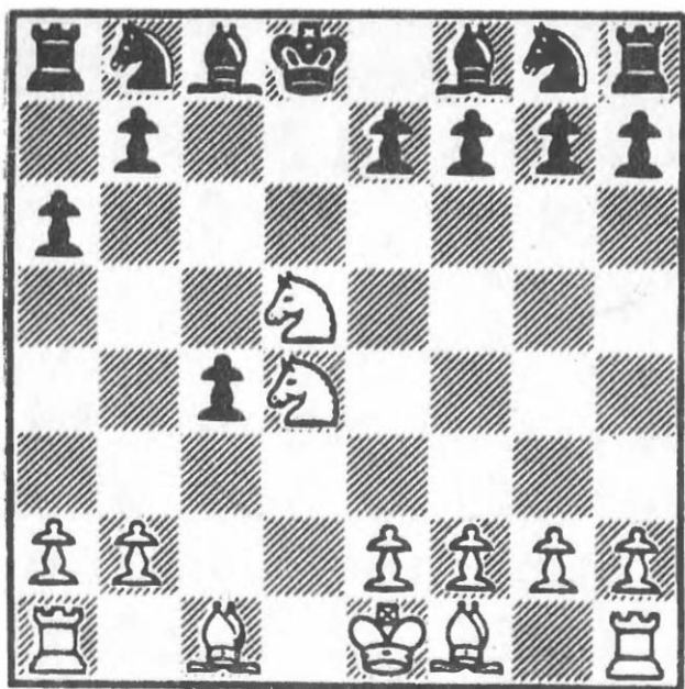
15 After 7...Kd8
